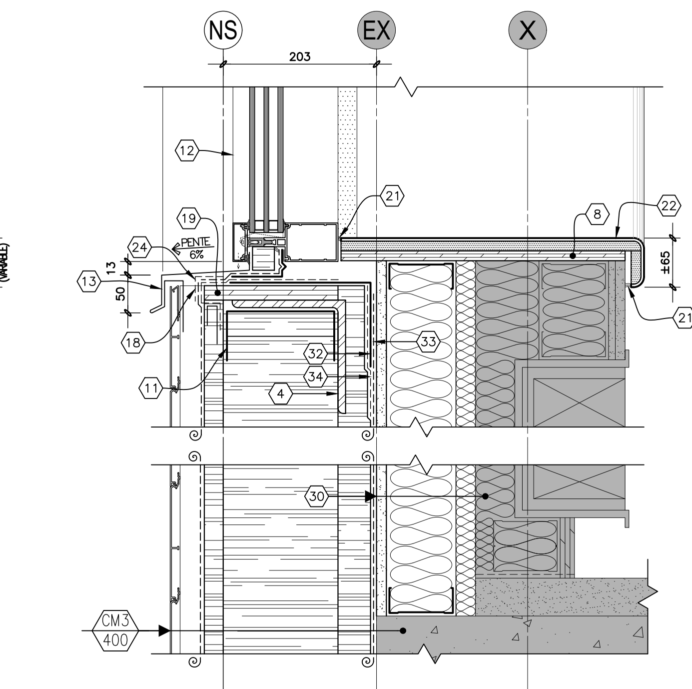
CONSTRUCTION
