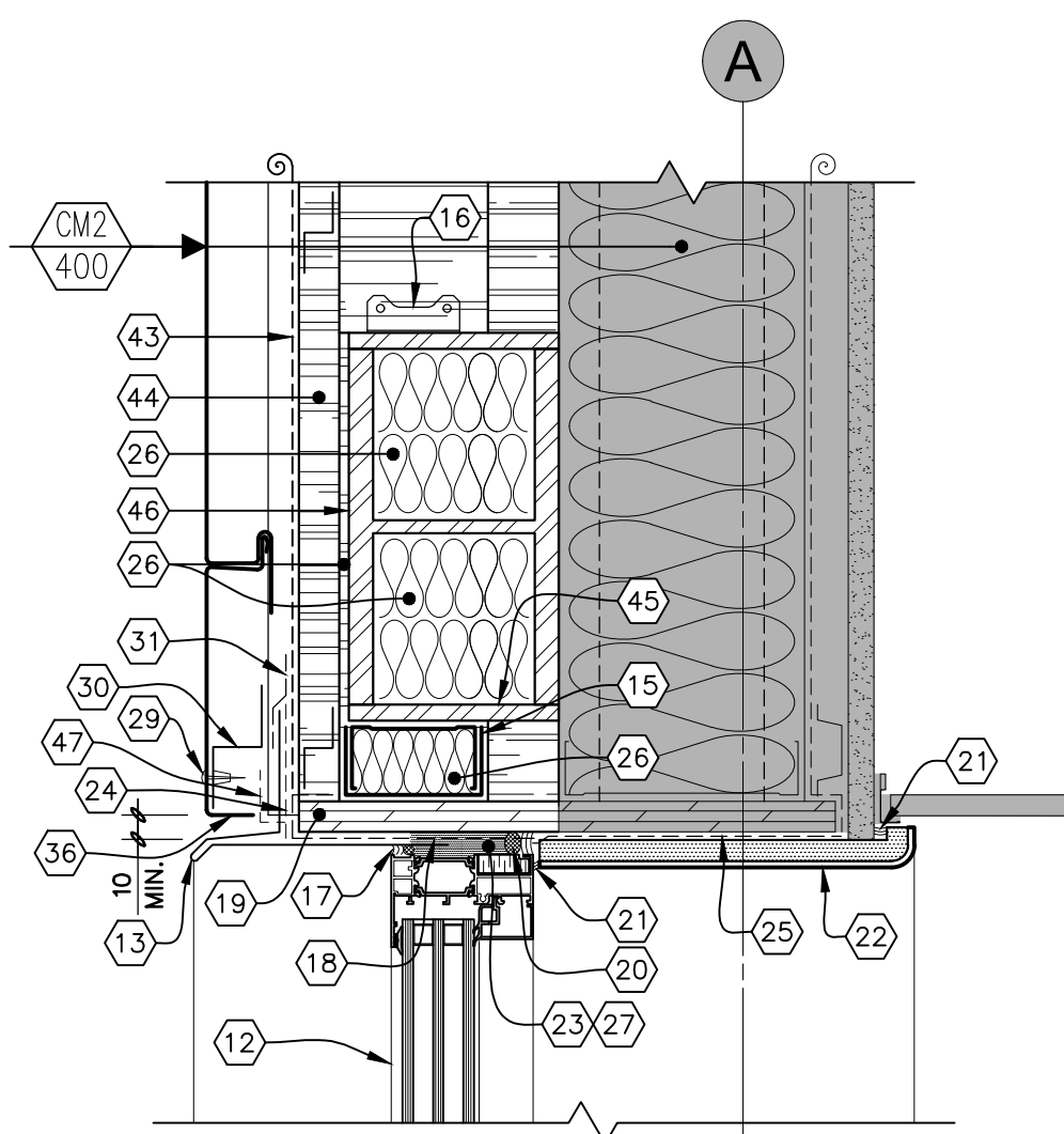
CONSTRUCTION
