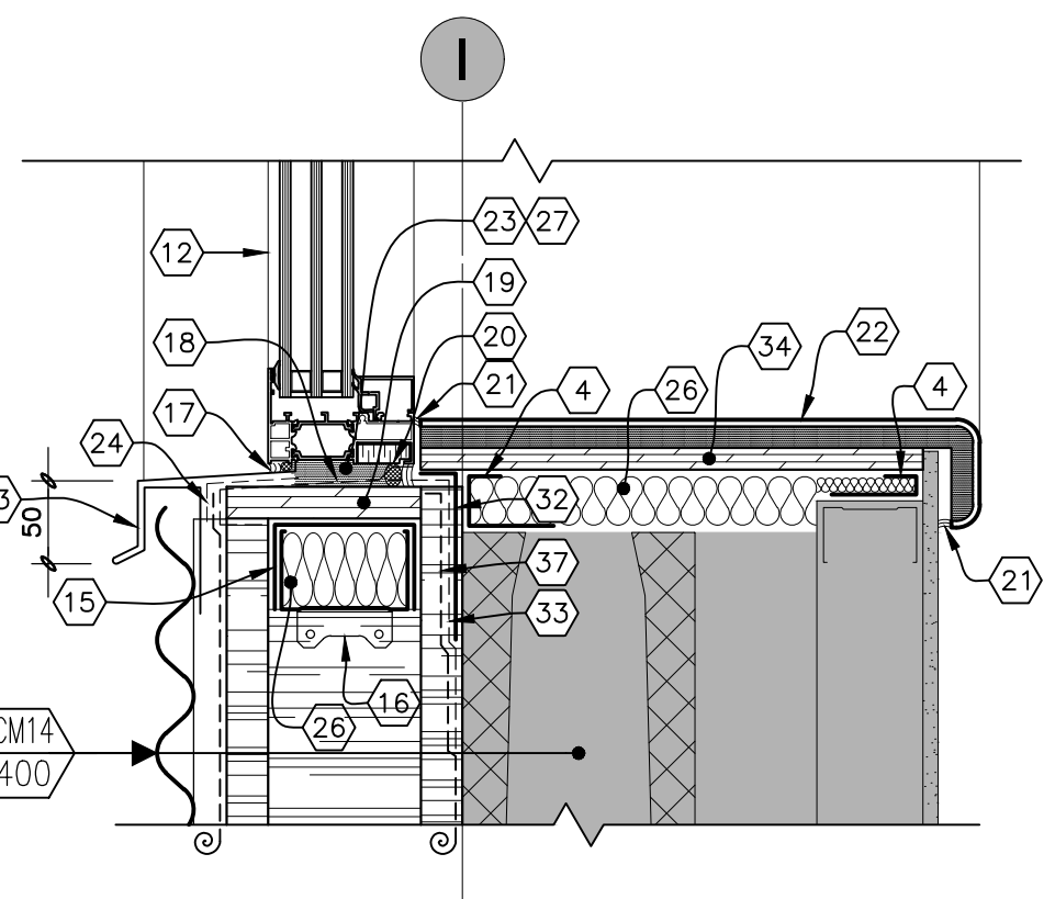
CONSTRUCTION
